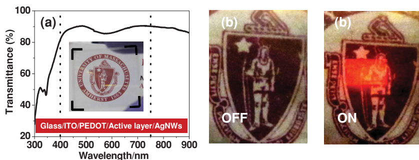
Figure 5. a) Transmission spectrum of the red transparent QD-LECs. The average transmittance in the visible region over 400 nm to 750 nm is 88%. The inset photograph shows the transparent QD-LECs. The black brackets indicate the border of the device. b) Photograph of the transparent QD-LECs in on and off states, demonstrating the uniformity of pixel illumination and device transparency.
