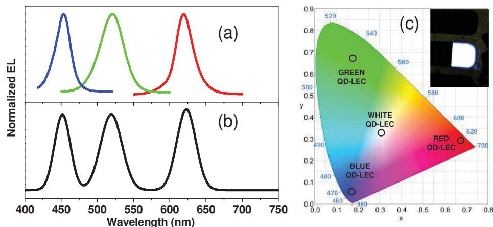
Figure 4. a) Normalized EL spectra of blue, green and red monochrome QD-LECs (blue, green, and red lines, respectively). b) EL spectrum for the white QD-LEC (@ 10 V). c) CIE chromaticity diagram indicating the color of blue, green, red, and white QD-LECs. Inset: photograph of a white QD-LEC in operation with 10 V of applied forward bias with CIE (0.33, 0.33).
